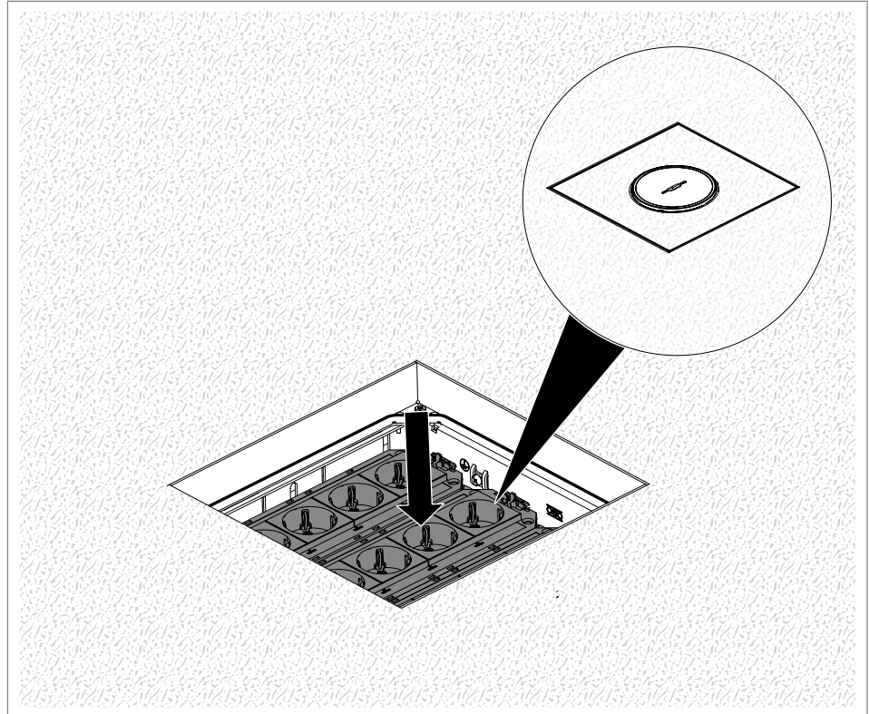
Fig. 18: Inserting accessories
