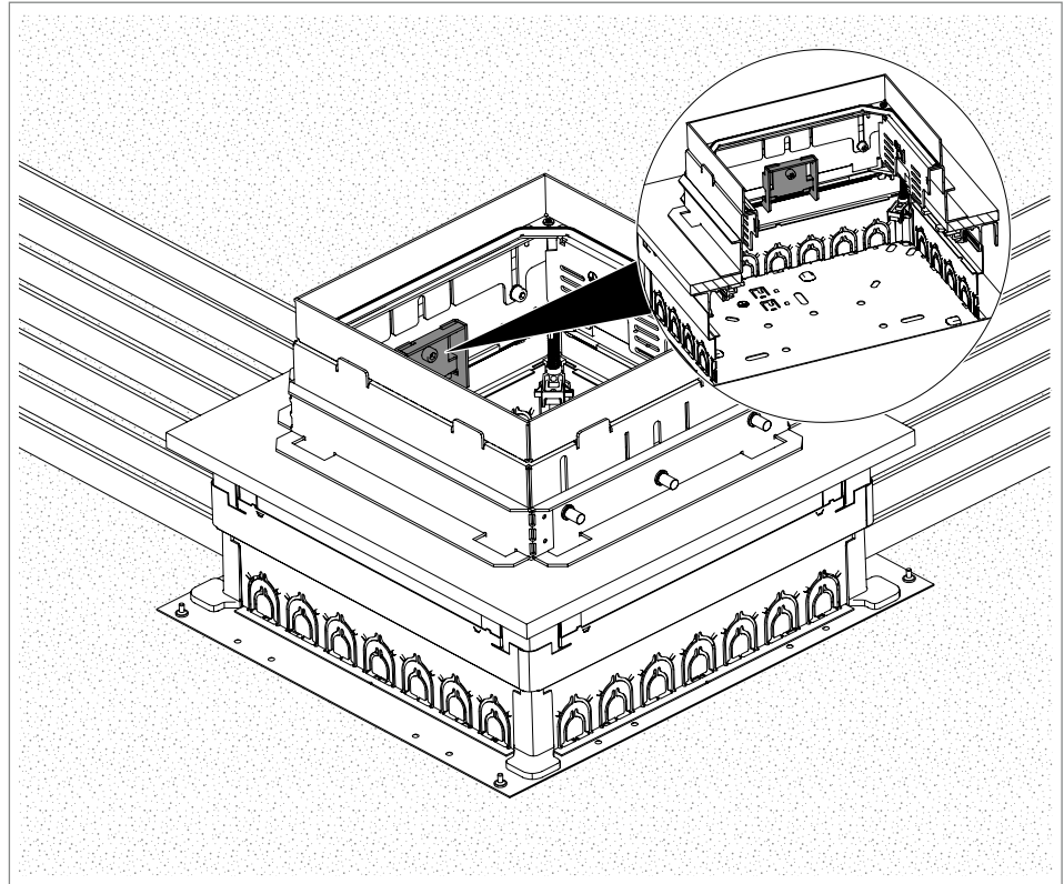
Fig. 9: Fastening the holding claws
