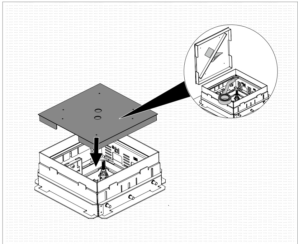
Fig. 13: Mask the cassette and screed protection cover
