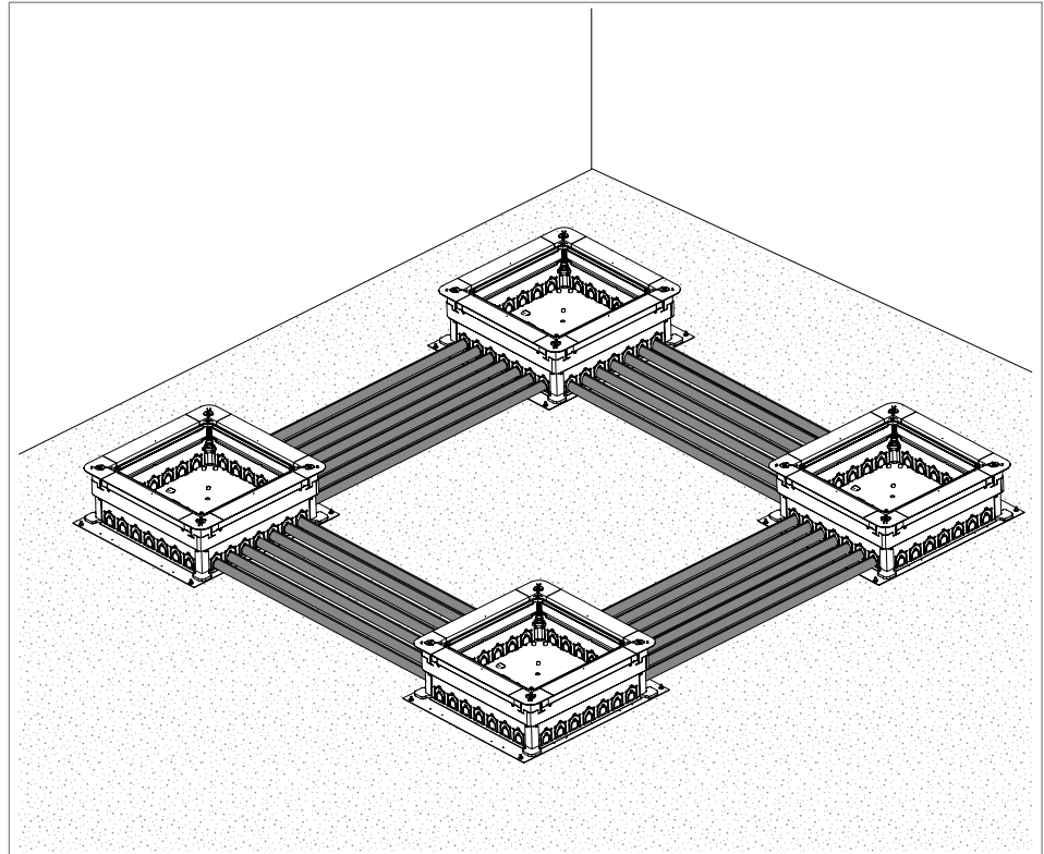
Fig. 5: Connecting the UZD/UGD55 underfloor accessory socket
