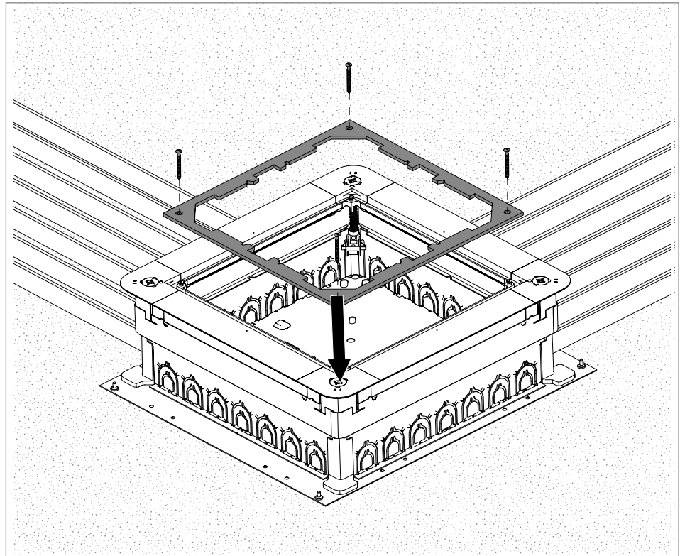
Fig. 7: Applying the mounting frame
