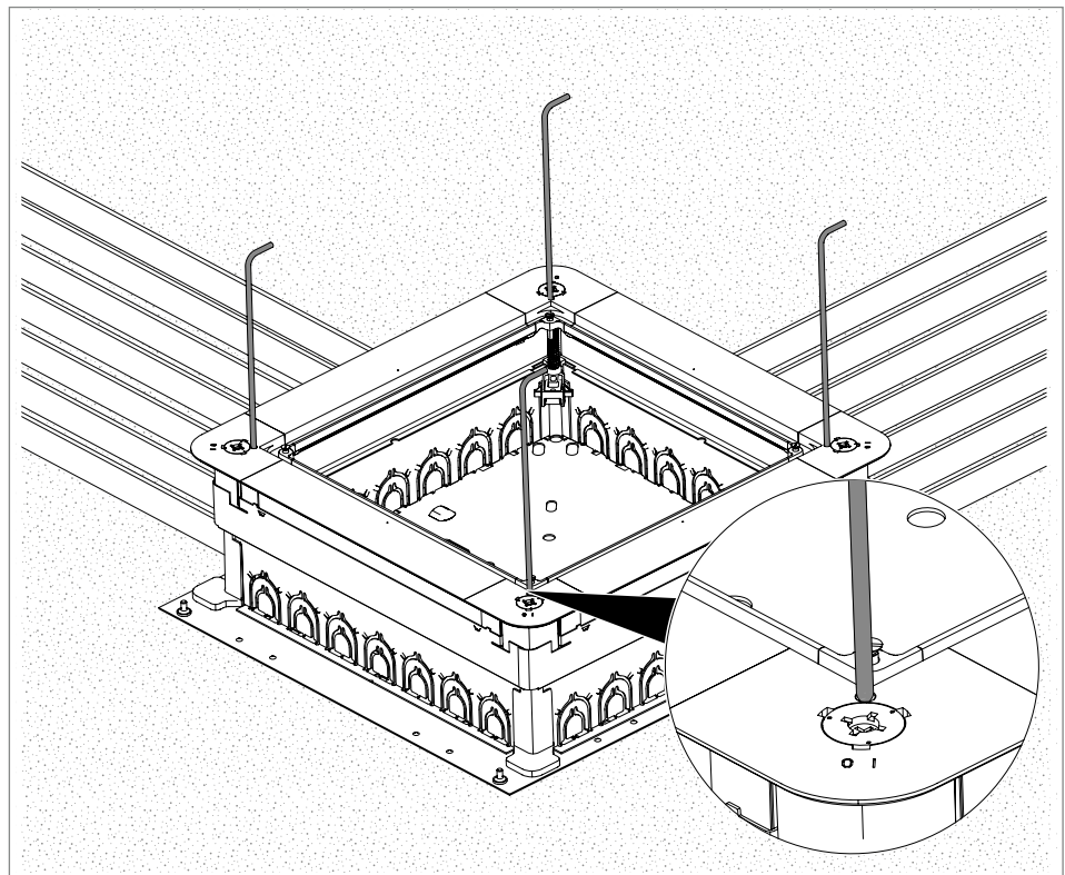
Fig. 6: Adjusting the height of the UZD/UGD55 underfloor accessory socket
