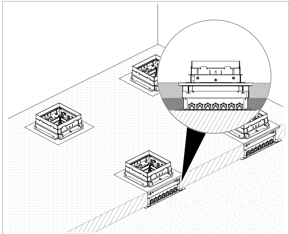
Fig. 12: Inserting the insulation/footfall sound insulation
