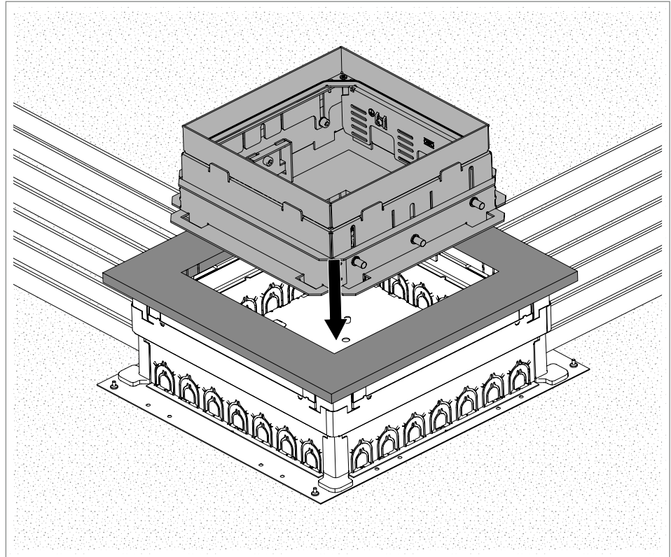
Fig. 8: Applying the ISO apron and cassette
