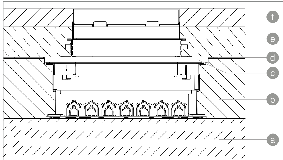
Fig. 2: Installation principle
