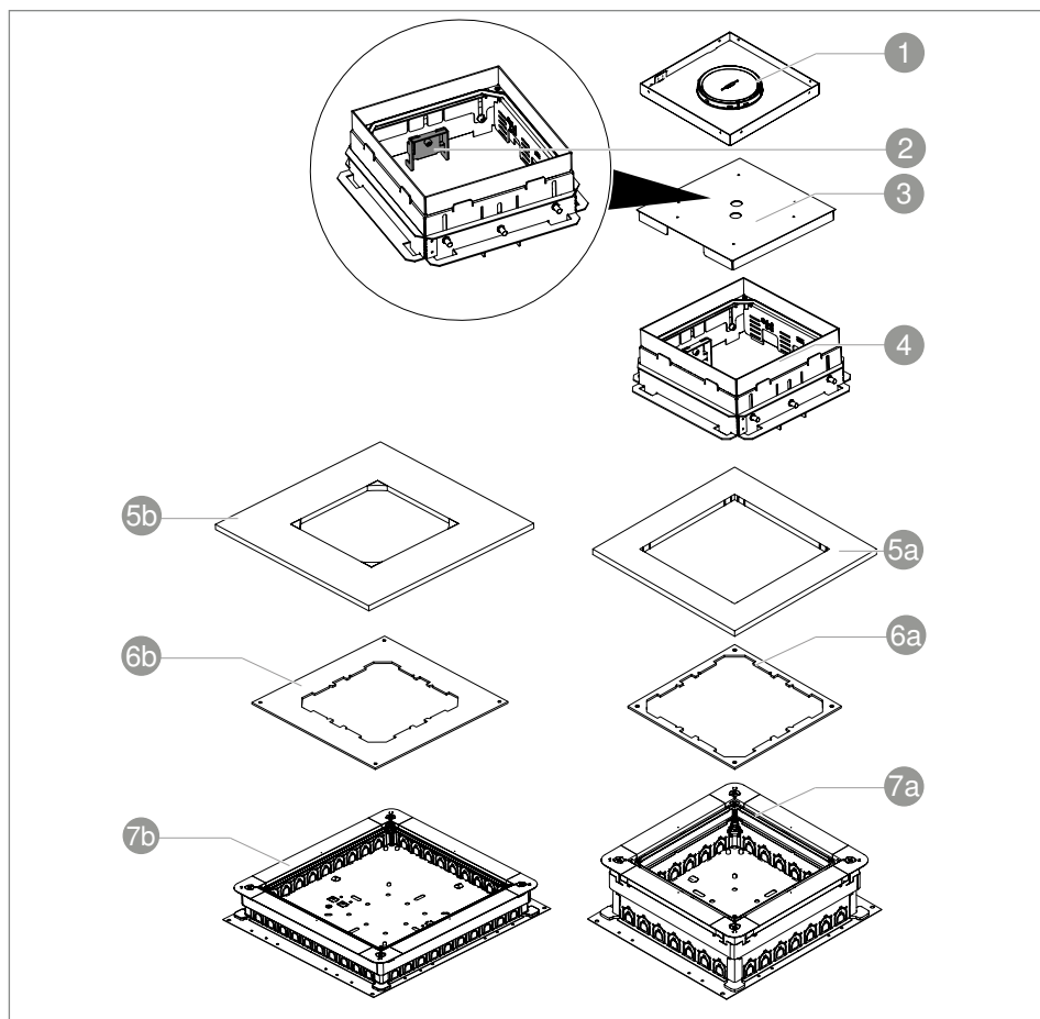
Fig. 1: Product description
