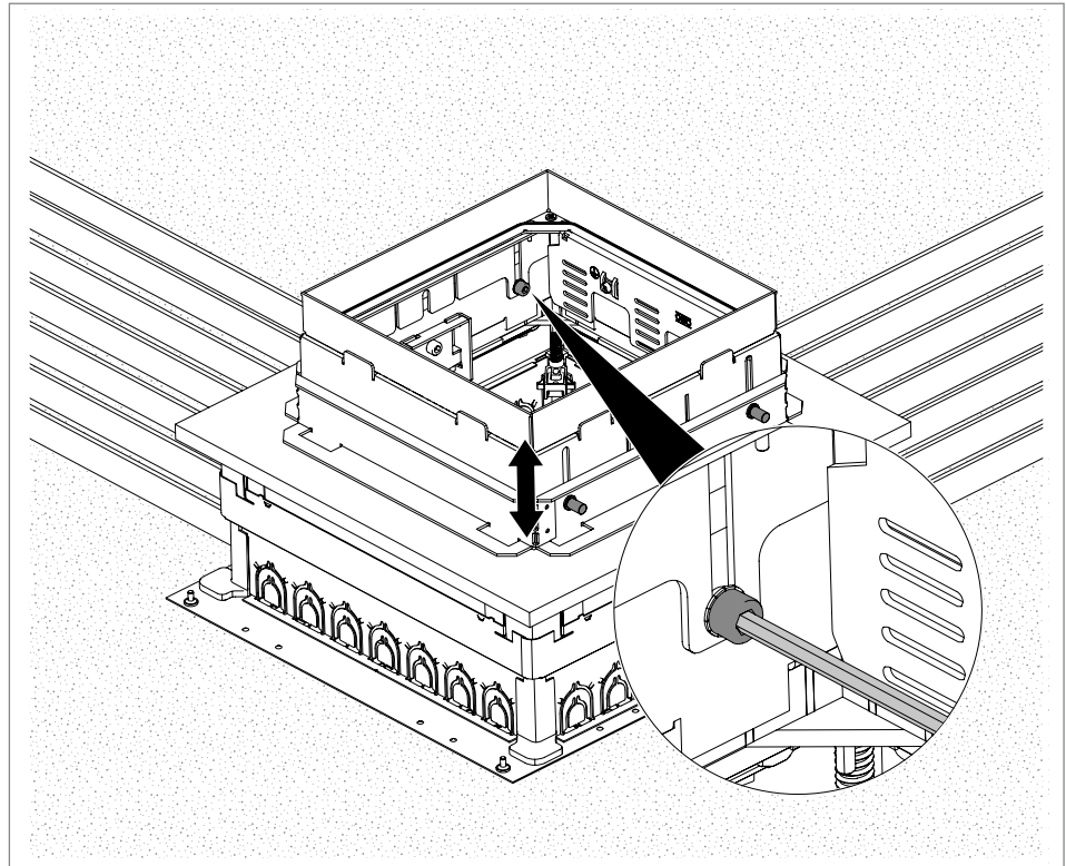
Fig. 11: Fine adjustment of the cassette
